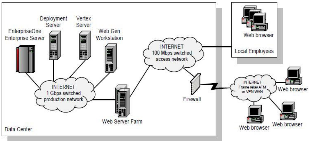
Sample EnterpriseOne Architecture Diagram
